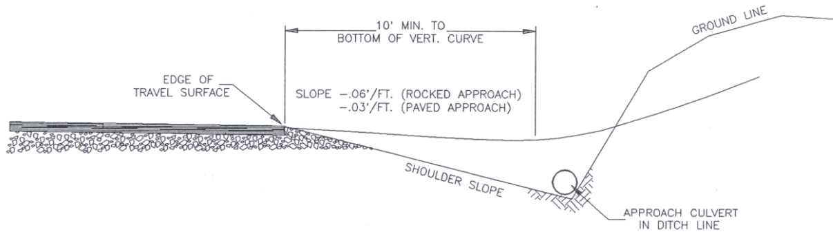
- CUT SECTION -
